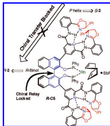
Figure 4. Atropisomeric nature of binaphthyl core locks axial chirality of central core in ( R )- C5 , which precludes relay of dendron helicity to catalytic center.
