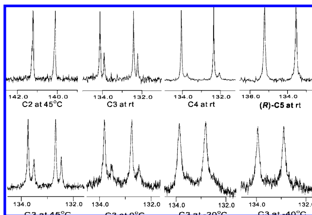
Figure 5. Top: ^{31}\text{P} NMR spectra of C2 – C5 . Bottom: Temperature-dependent spectra of C3 .
